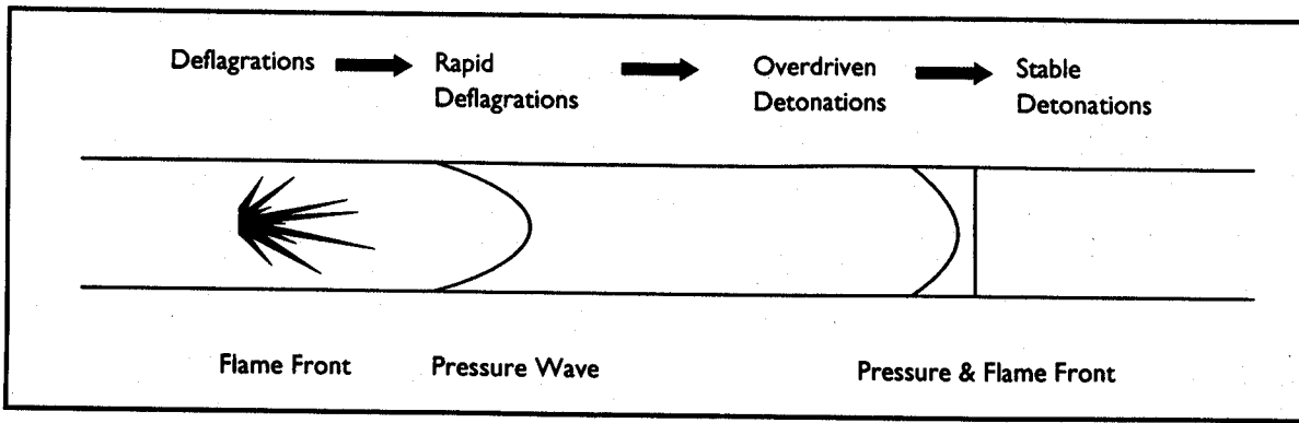
Figure 2: Explosion Phenomena In Pipes
