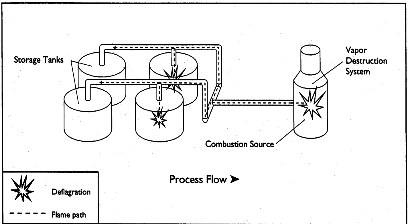
Figure 1: Unprotected Vapor Collection System
