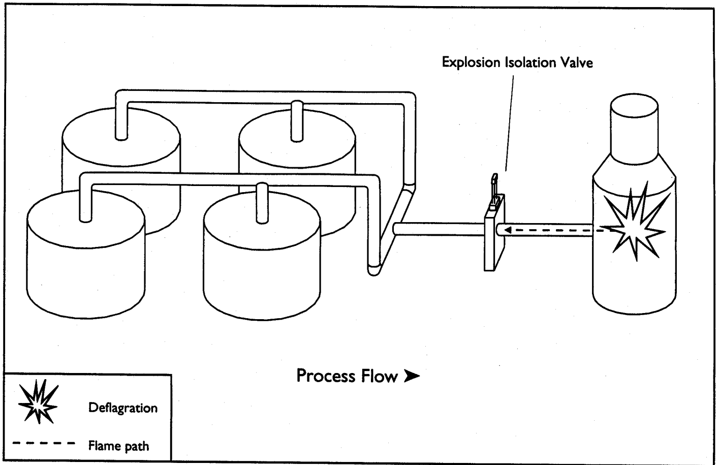
Figure 4: Protected Vapor Recovery System
