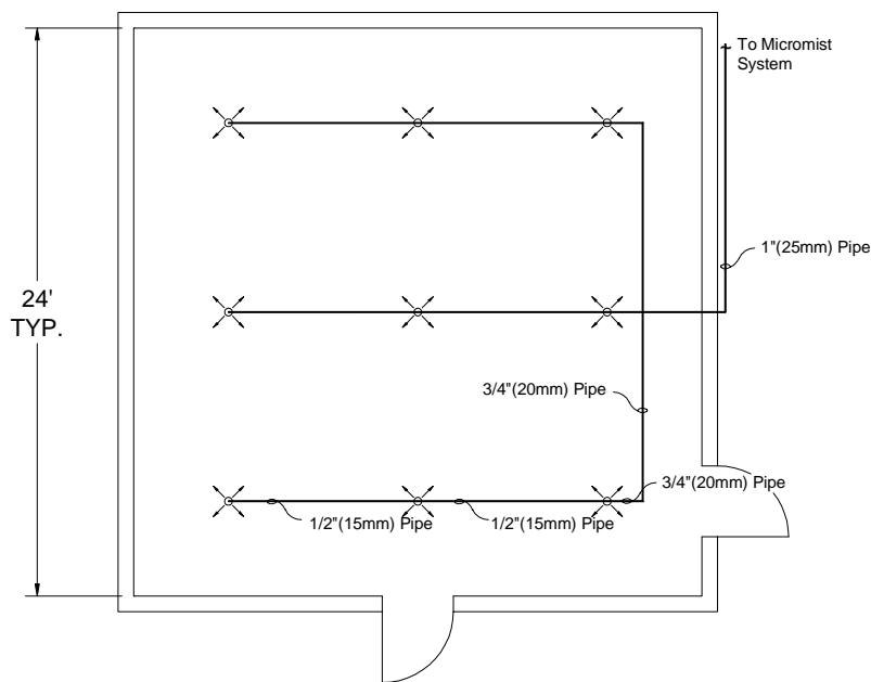
Typical Piping Layout Machinery Space
