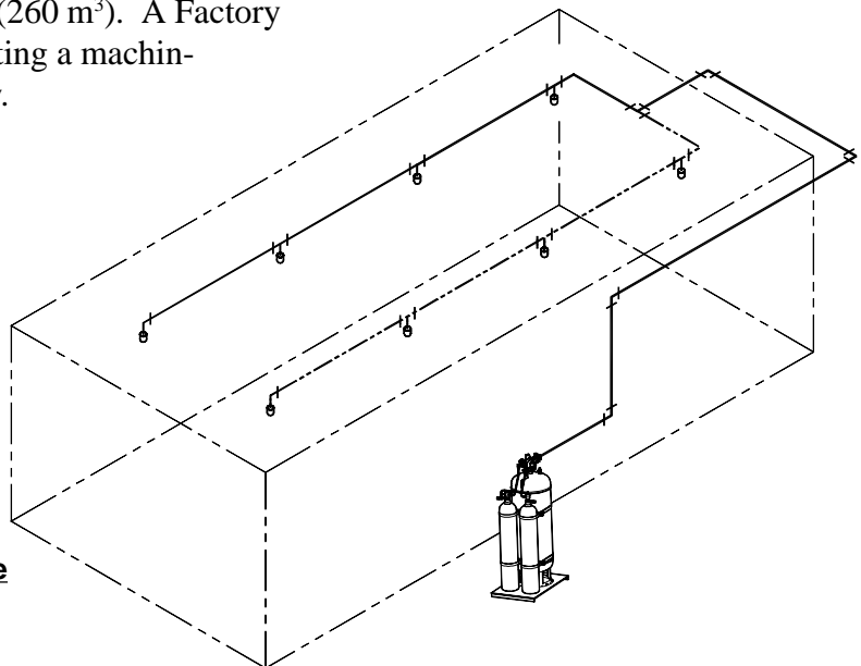
“Machinery Space” Protected by a Fike Micromist Extinguishing System
