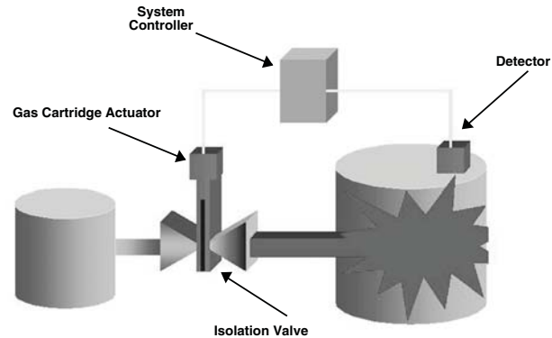
Schematic of Explosion Isolation System. Detector senses onset of deflagration, sends signal to control panel which in turn closes valve and stops flame and pressure transmission
